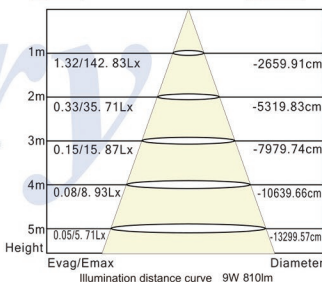
Illumination distance curve 9W 810lm
