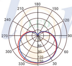
Light Distribution Curve 9W 810lm
